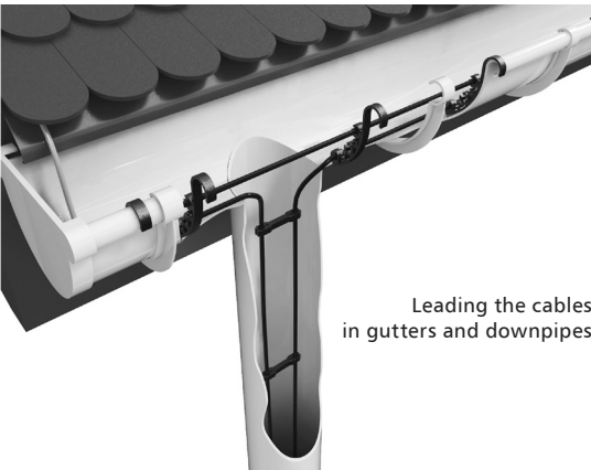
Downpipe spacing wire with clips DSW-2
