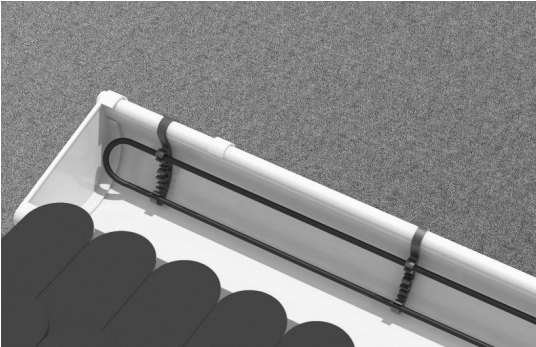
Gutter holder GH-2
